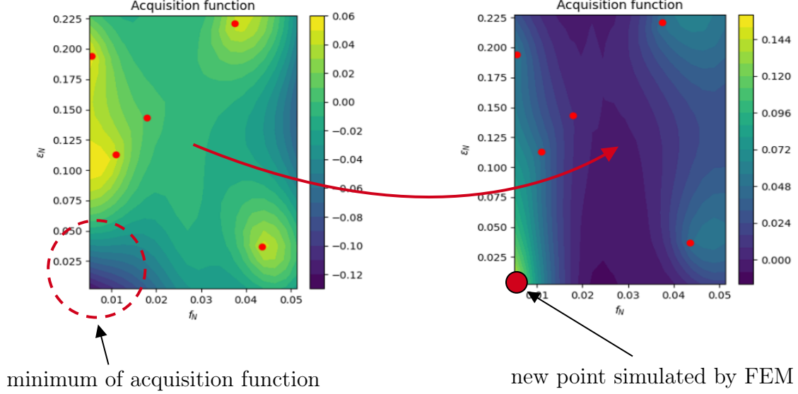
Figure 2: Choice of the new pair of GTN parameter f_N and \varepsilon_N for an additional FEM simulation.
